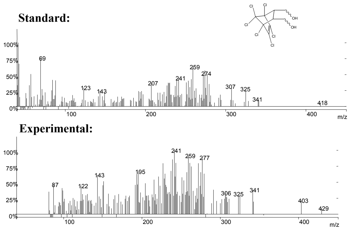
Sup. Figure 4. Mass spectra of ES diol.
